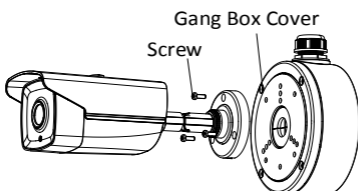
Figure 2-11 Fix the Camera with the Gang Box
