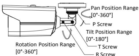
Figure 2-9 3-axis Adjustment
