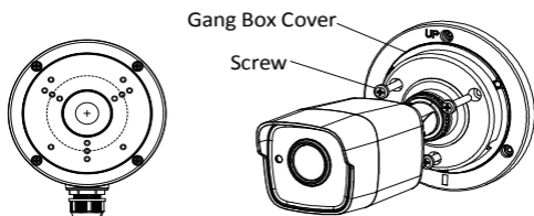
Figure 2-4 Fix the Camera with the Gang Box
